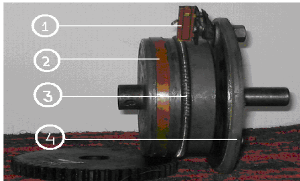
Fig.5. INPUT TORQUE METER Carbon brush holder (2) Copper ring (3) Resistance wire (nichrome wire) (4) Cover plate
