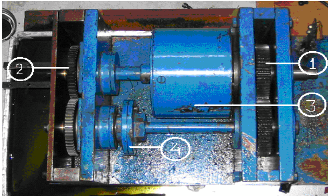
Fig. 1. GEAR TESTING MACHINE
