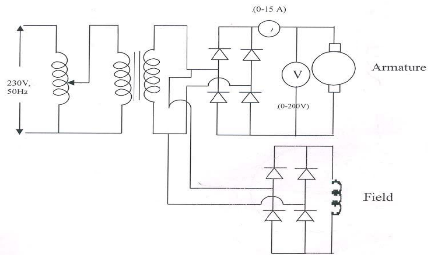
Fig. 8. Illustrates the separate excitation of the field and power supply to the armature.
