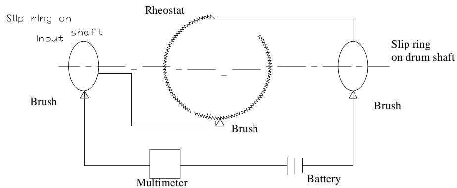
Fig.7. Circuit diagram to measure power loss at input Torque meter.
